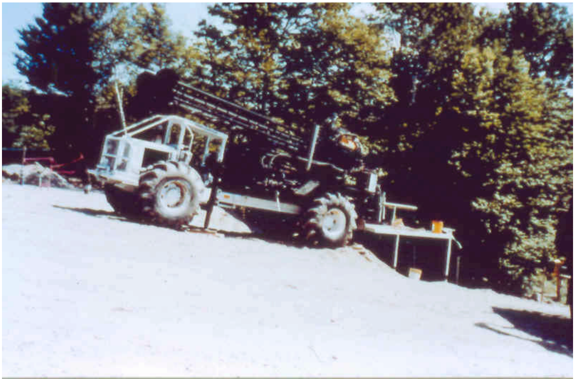
Photograph 4a – Low pressure and flotation tire mounted ATV rig.
